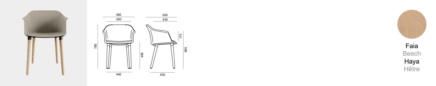
C Piramidal (madeira) - Pyramidal (wood) - Piramidal (madera) - Pyramidal (bois)
