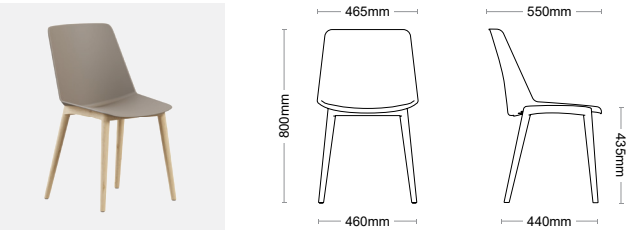
K 4 pés (madeira) - 4 leg (wood) 4 pies (madera) - 4 pieds (bois)
