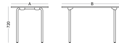
Mesa empilhável - Stackable table - Mesa apilable - Table empilable
